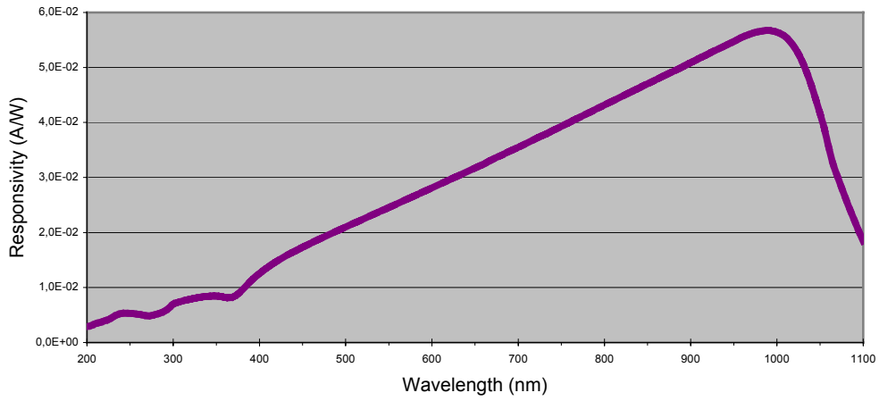
PD50-D9-UV Spectral Responsivity General Absorption Curves
