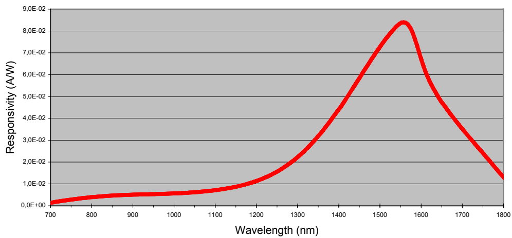
PD50-D9-IR Spectral Responsivity
