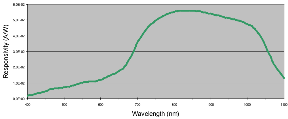
PD50-D9-VIS Spectral Responsivity
